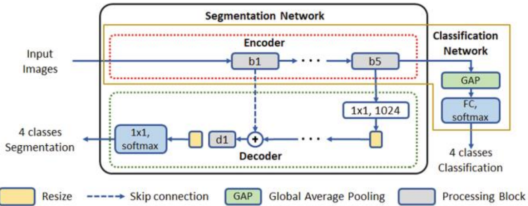
Fig. 1. Overview of the proposed approach. A classification network consists of an encoder and two processing layers. A segmentation network contains an encoder and decoder.
